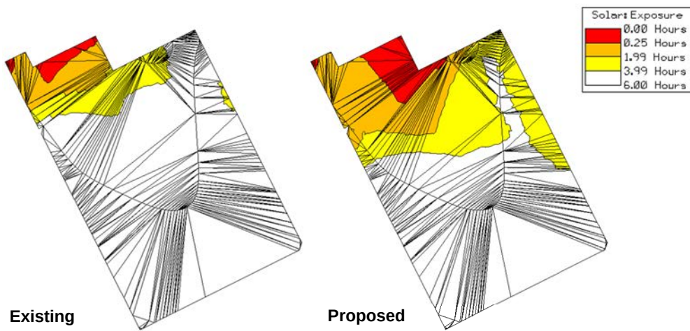
Figure 206 – solar insolation to Mary Ann Street Park
